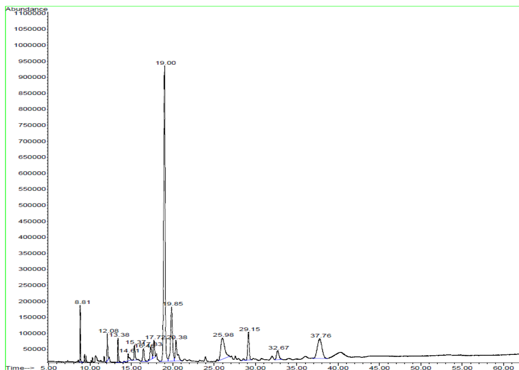
Appendix 1. GC chromatogram of S. platystegia essential oil
